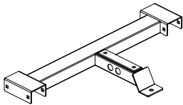
① Foot Plate Bottom Frame 1x
